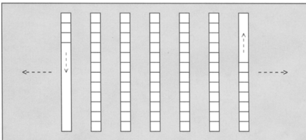
Figure 6.3. Internal Structure of a Deque
